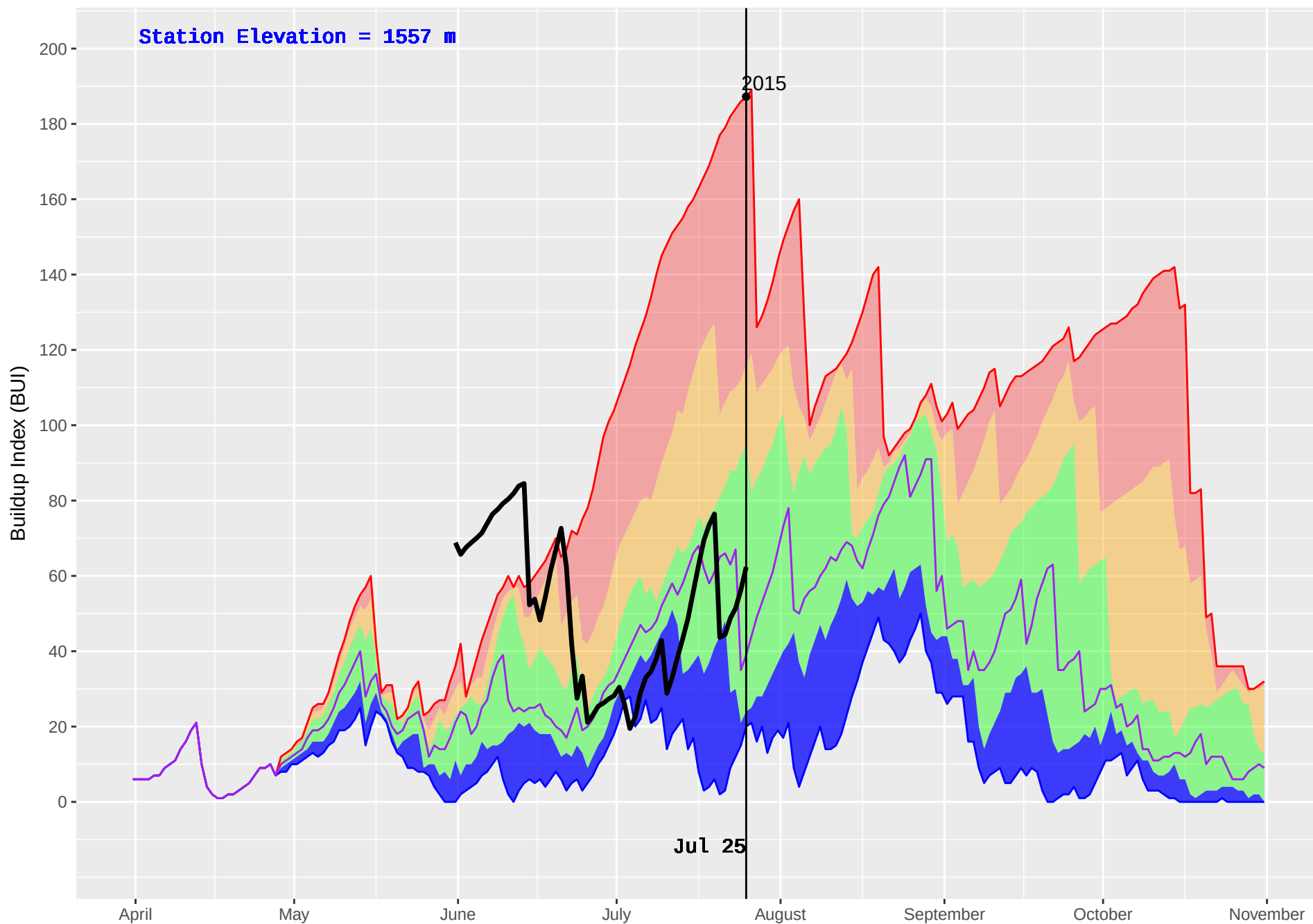
SKOONKA (1024) : Historical (2008–2016) and Current (2018) Noon Buildup Index (BUI)
