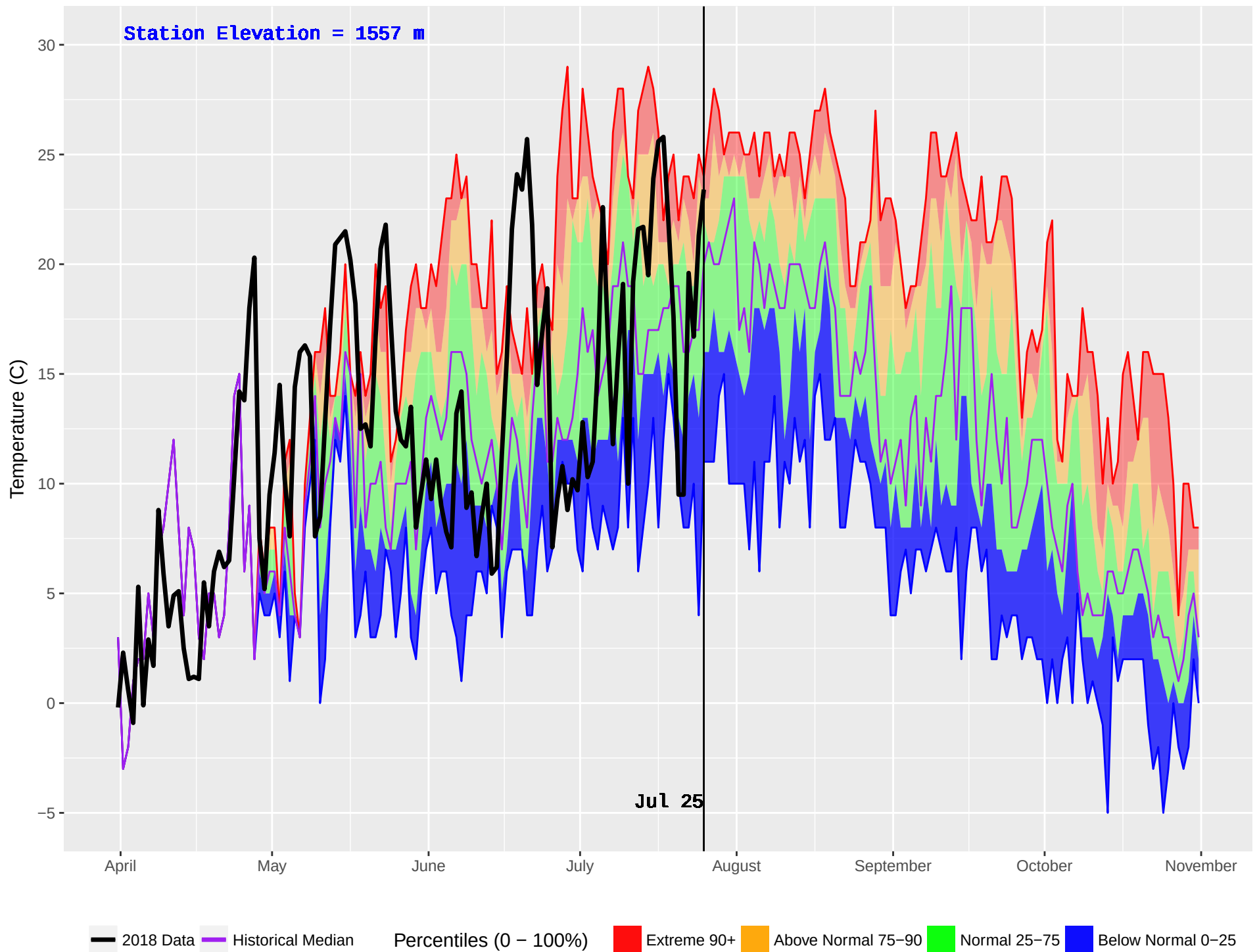
SKOONKA (1024) : Historical (2008–2016) and Current (2018) Noon Temperature
