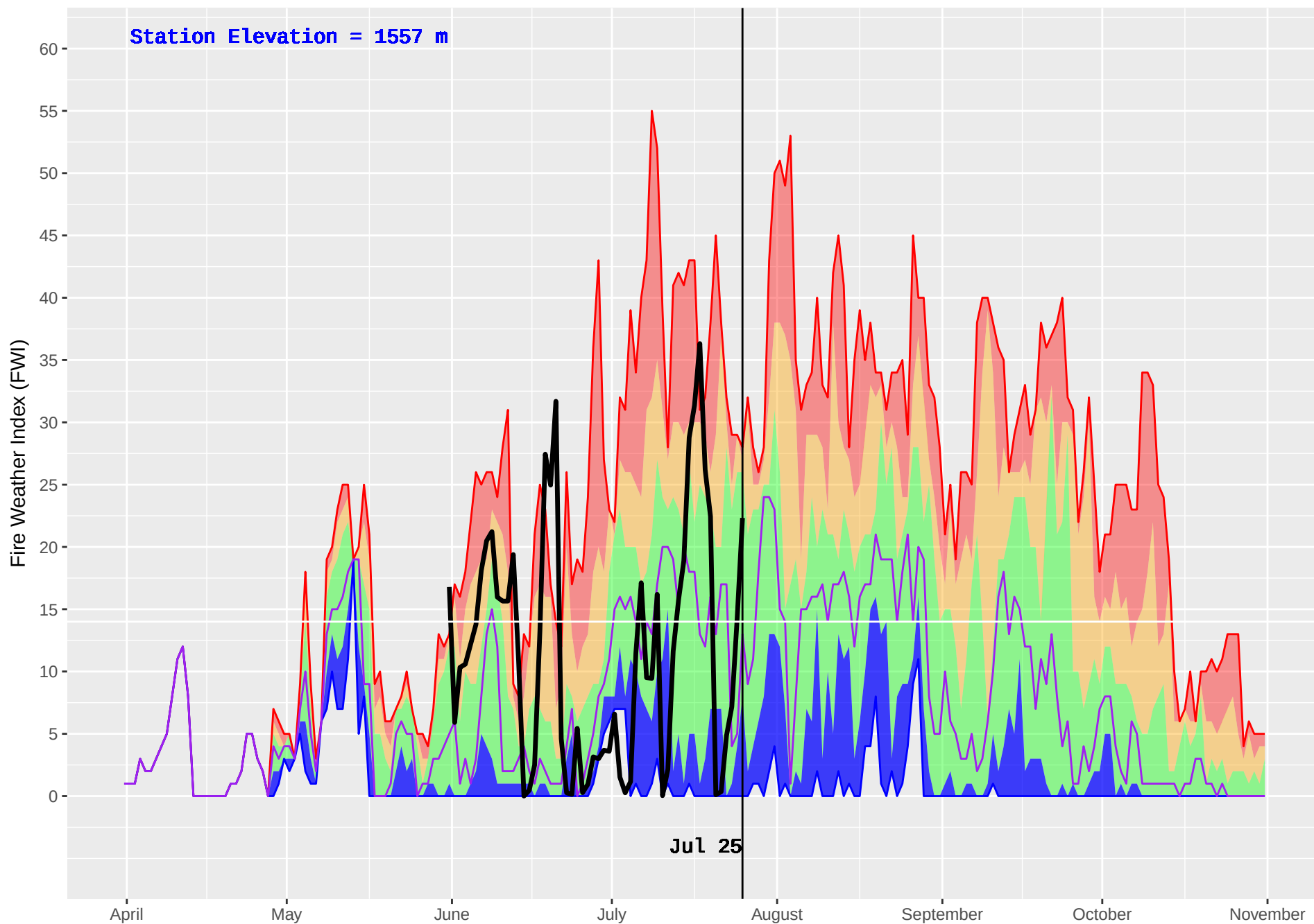
SKOONKA (1024) : Historical (2008–2016) and Current (2018) Noon Fire Weather Index (FWI)
