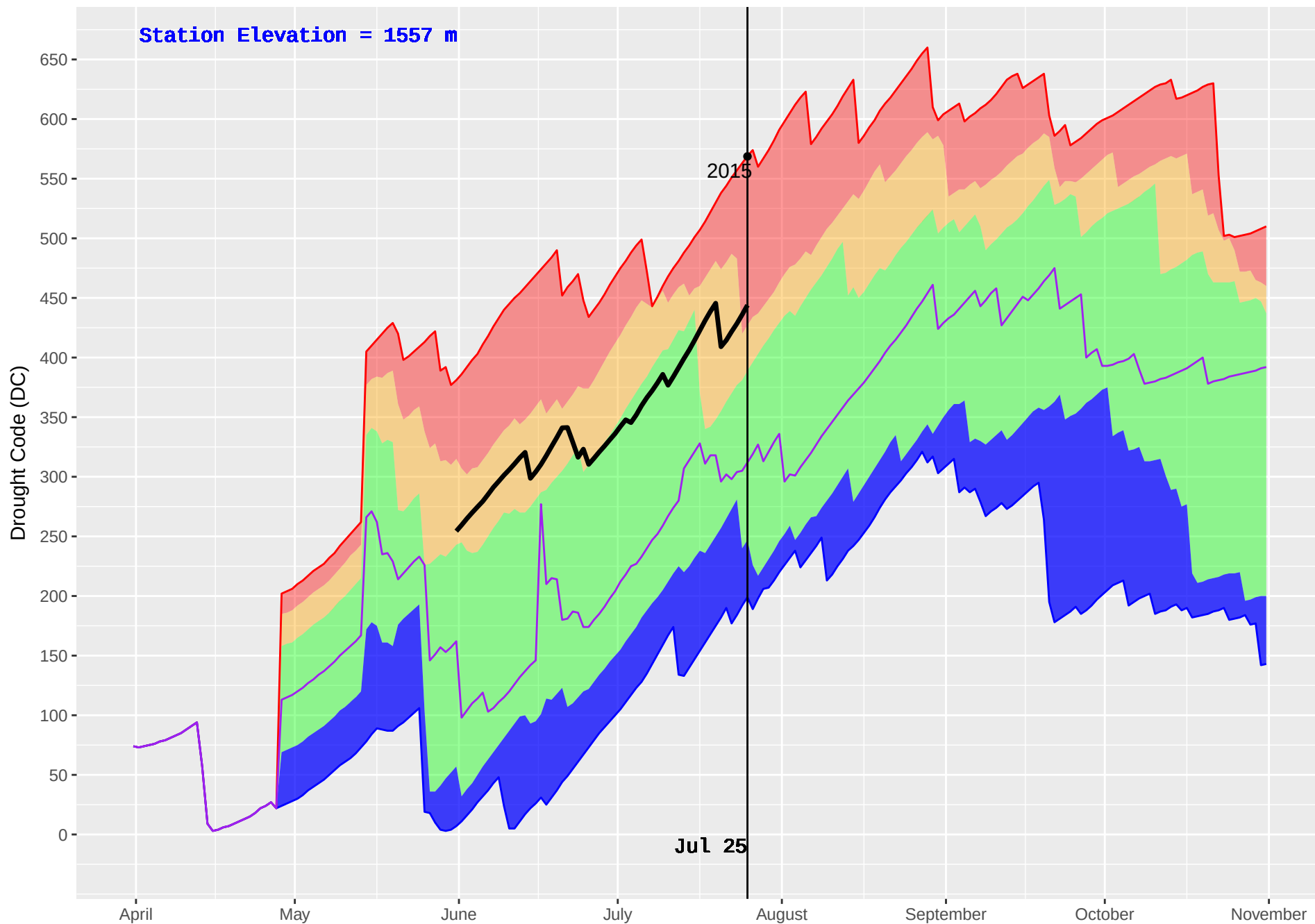
SKOONKA (1024) : Historical (2008–2016) and Current (2018) Noon Drought Code (DC)
