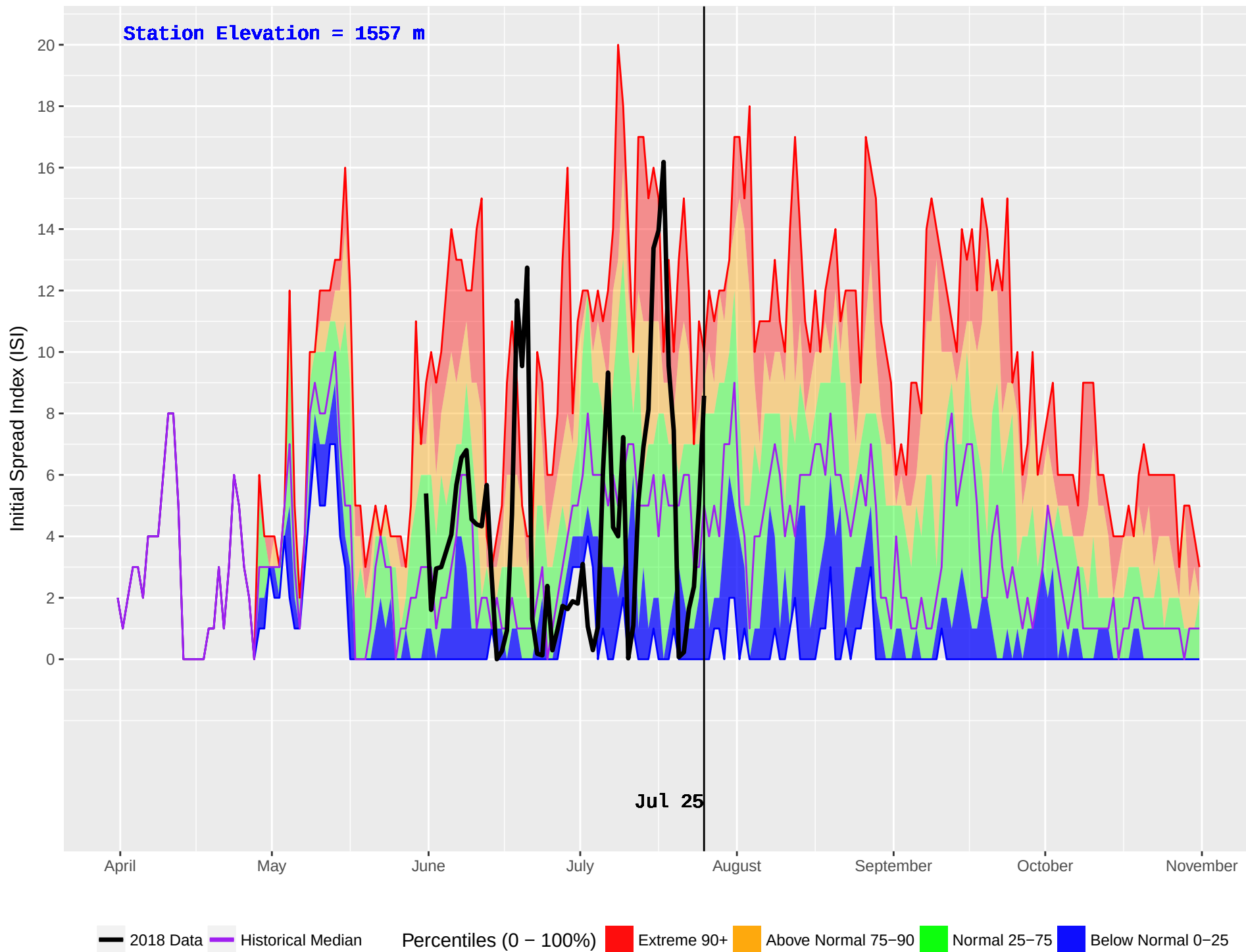
SKOONKA (1024) : Historical (2008–2016) and Current (2018) Noon Initial Spread Index (ISI)
